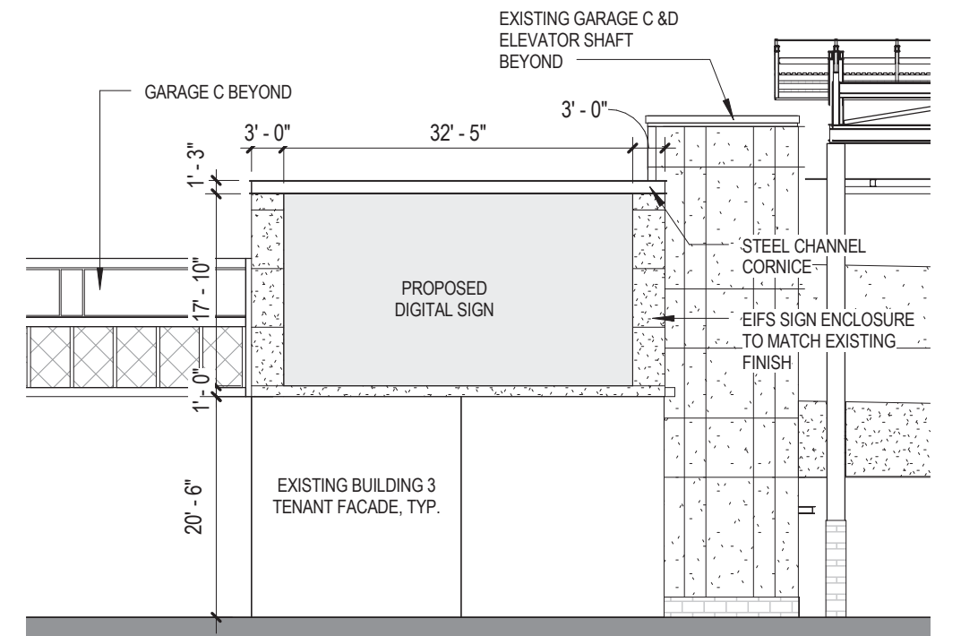
WEST ELEVATION - 1/16" = 1'-0"
