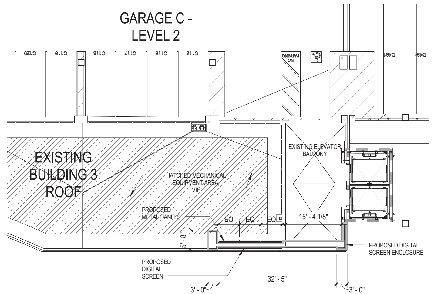
PLAN - 1/16" = 1'-0"
