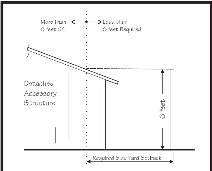
Side Yard Accessory Structure
